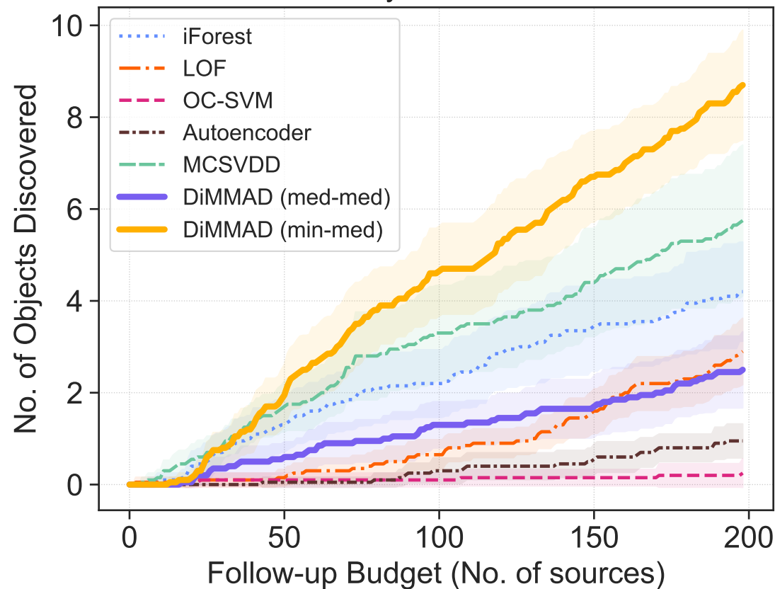
Anomaly: SLSN-I+host
